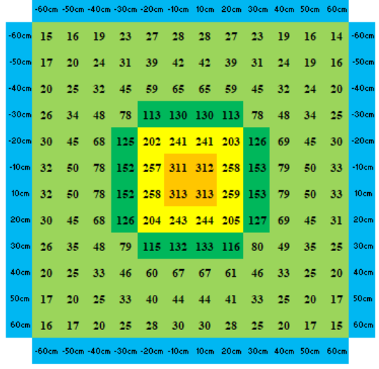
30cm height reflective mylar grow tent 1.2m x 1.2m
